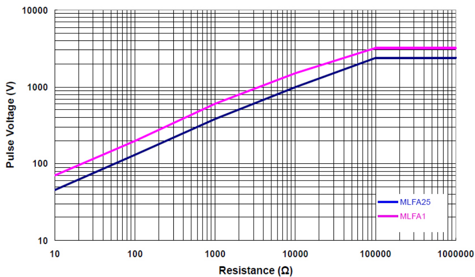
10 / 700 \mu s Lightning Surge
