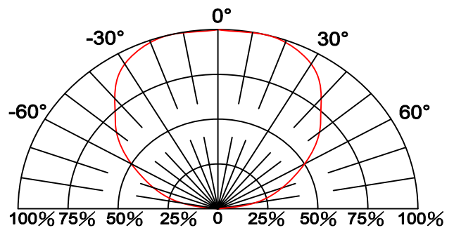
Fig.6 Directive Radiation
