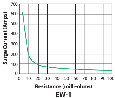
PULSE/SURGE CHART (Typically 50 msec duration)
